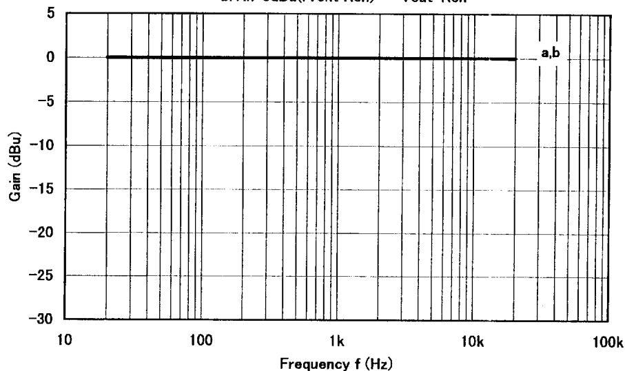
TruSurround GAIN STRUCTURE BYPASS Mode ( V^+=12V ) a: V_{in}=0dBu(\text{Front Lch}) \rightarrow V_{out}=Lch b: V_{in}=0dBu(\text{Front Rch}) \rightarrow V_{out}=Rch
