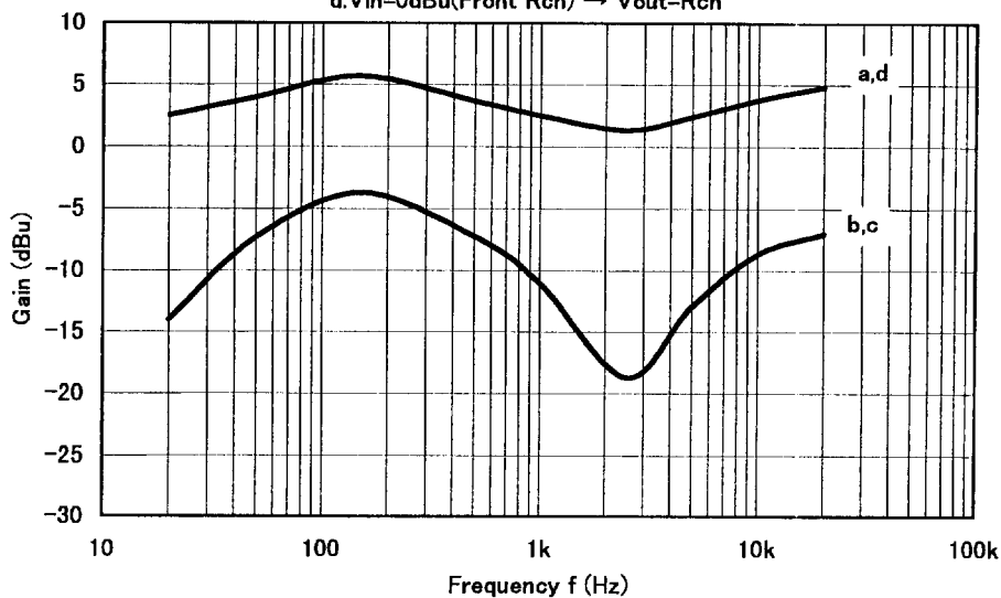
TruSurround (Lt/Rt) GAIN STRUCTURE Tru Mode ( V^+=12V ) a: V_{in}=0dBu(\text{Front Lch}) \rightarrow V_{out}=Lch b: V_{in}=0dBu(\text{Front Lch}) \rightarrow V_{out}=Rch c: V_{in}=0dBu(\text{Front Rch}) \rightarrow V_{out}=Lch d: V_{in}=0dBu(\text{Front Rch}) \rightarrow V_{out}=Rch
