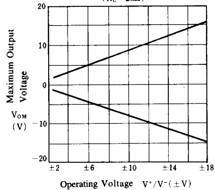
Maximum Output Voltage vs. Operating Voltage
