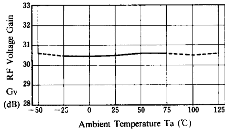
RF Voltage Gain vs. Temperature
