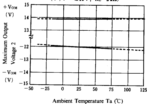
Maximum Output Voltage 2 vs. Temperature
