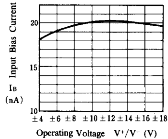
Input Bias Current vs. Operating Voltage
