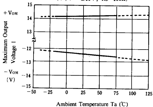
Maximum Output Voltage 1 vs. Temperature
