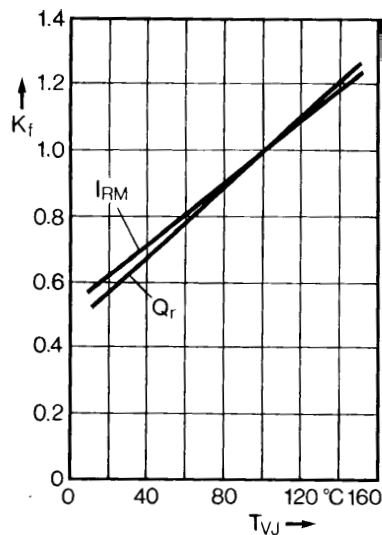
Fig. 14. Dynamic parameters versus junction temperature.
