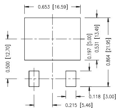
Min. Recommended Footprint
