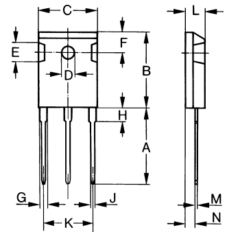
TO-247 AD (IXFH) Outline
