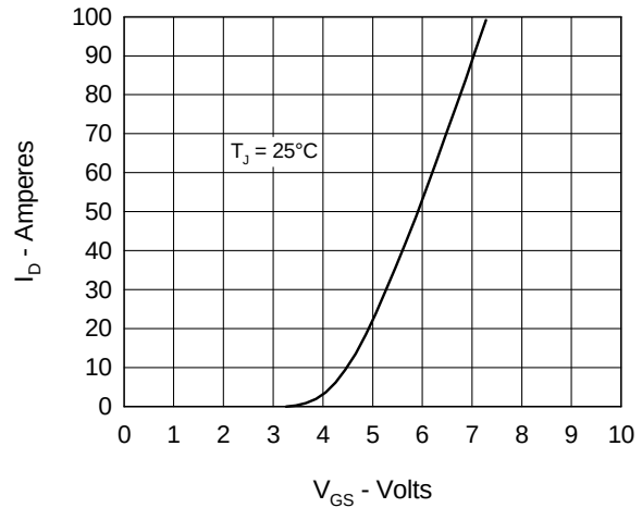
Fig. 2 Input Admittance
