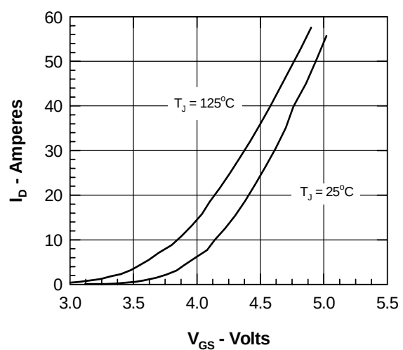
Figure 6. Admittance Curves
