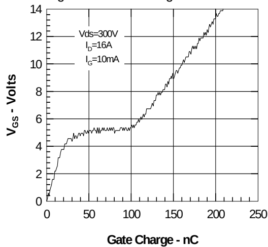
Figure 7. Gate Charge
