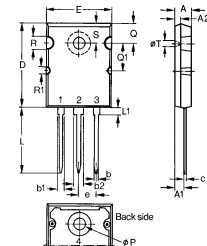
TO-264 AA (IXFK) Outline
