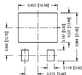
Min. Recommended Footprint
