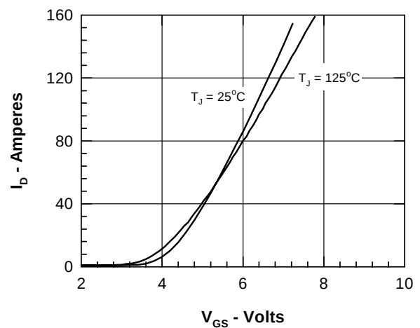
Figure 6. Admittance Curves
