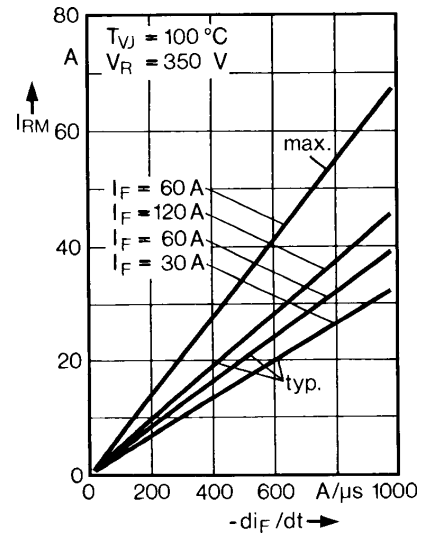
Fig. 13. Peak reverse current vs. -di_F/dt .
