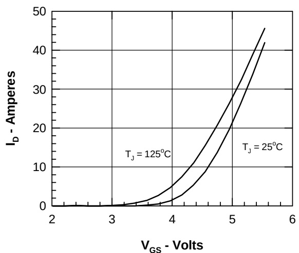
Figure 6. Admittance Curves
