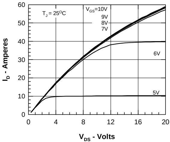
Fig.1 Output Characteristics
