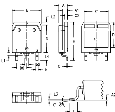
TO-268AA (IXFT) (D 3 PAK)
