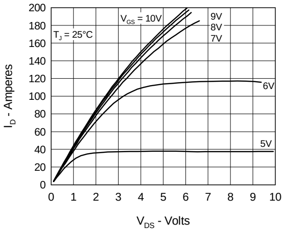
Fig. 1 Output Characteristics
