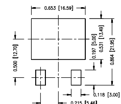
Min. Recommended Footprint
