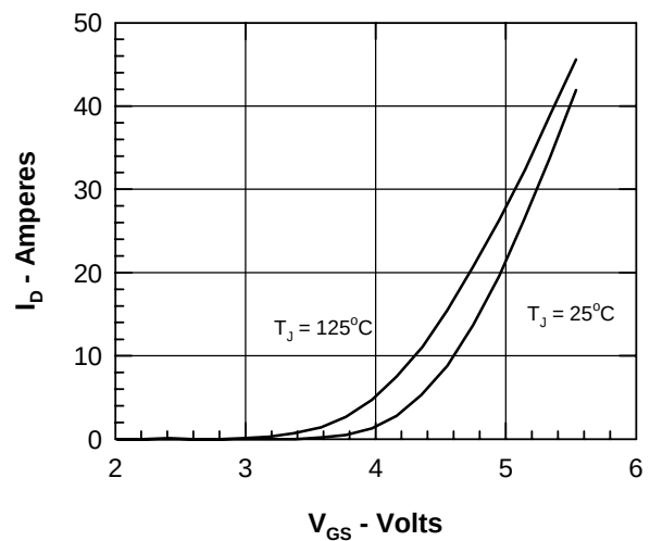
Figure 6. Admittance Curves
