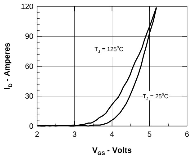
Figure 6. Admittance Curves
