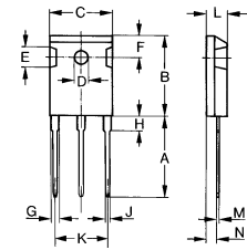
TO-247 AD (IXFH) Outline
