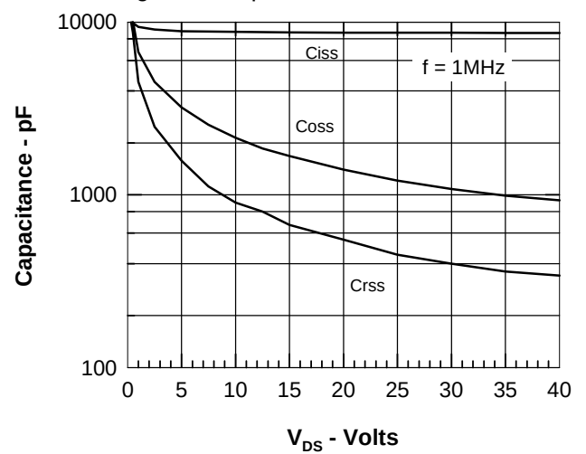
Figure 8. Capacitance Curves
