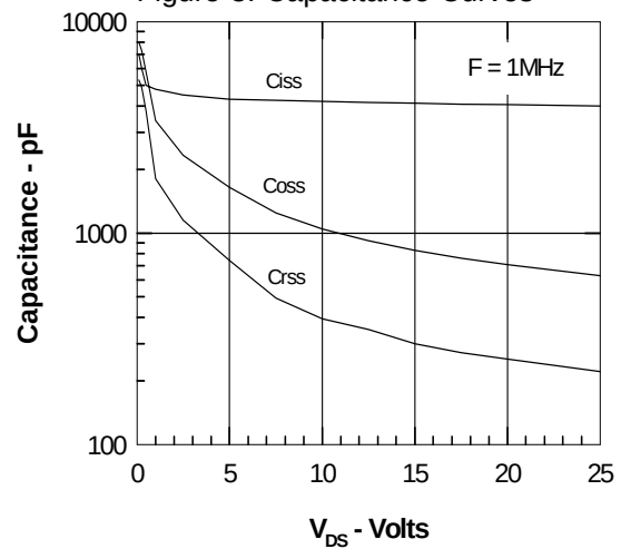
Figure 8. Capacitance Curves
