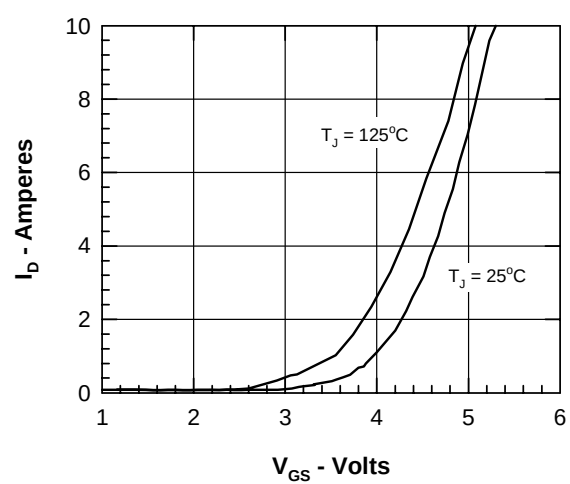
Figure 6. Admittance Curves
