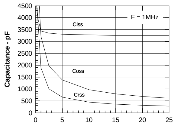
Figure 8. Capacitance Curves
