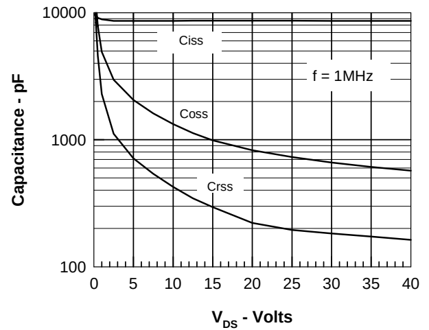
Figure 8. Capacitance Curves
