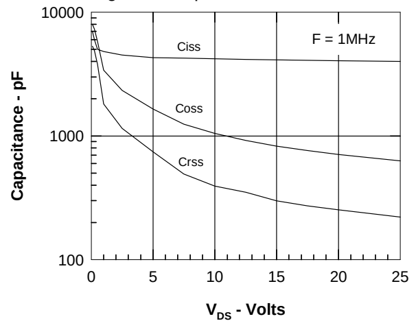
Figure 8. Capacitance Curves
