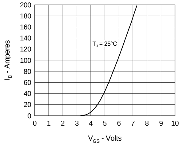
Fig. 2 Input Admittance
