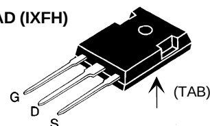
TO-204 AE (IXFM)
