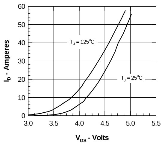
Figure 6. Admittance Curves
