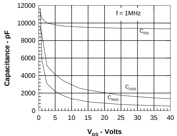
Figure 8. Capacitance Curves
