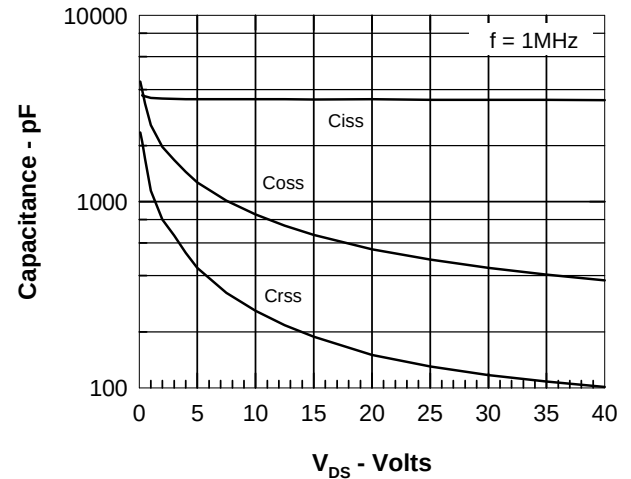
Fig.8 Capacitance Curves
