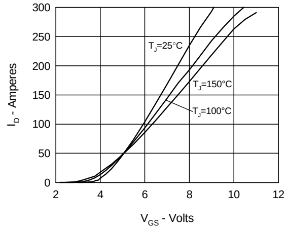
Fig. 2 Input Admittance
