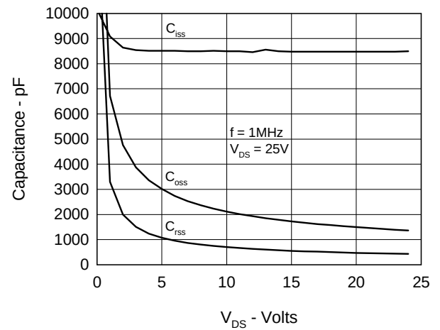
Fig.8 Capacitance Curves
