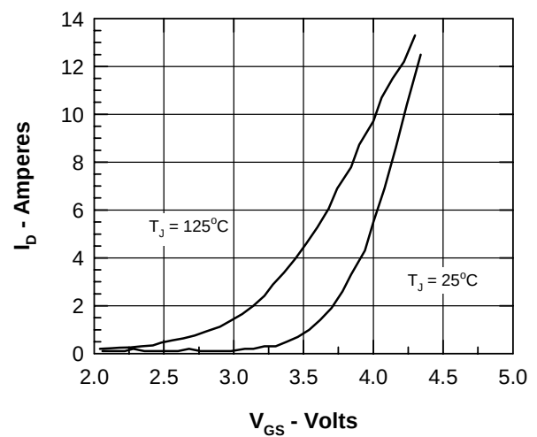
Fig.6 Input admittance
