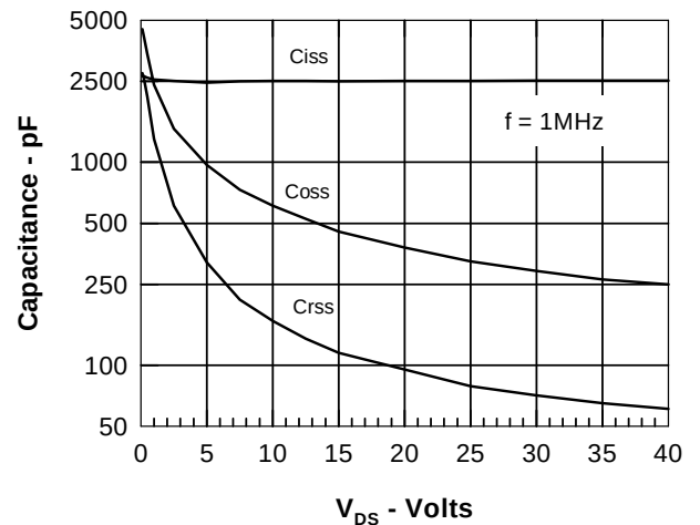
Figure 8. Capacitance Curves
