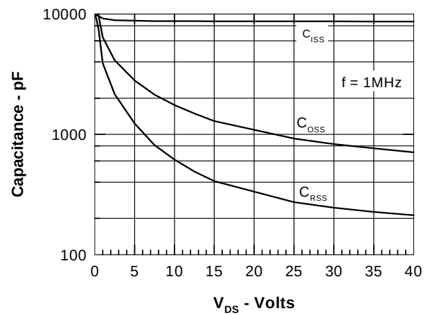
Figure 8. Capacitance Curves
