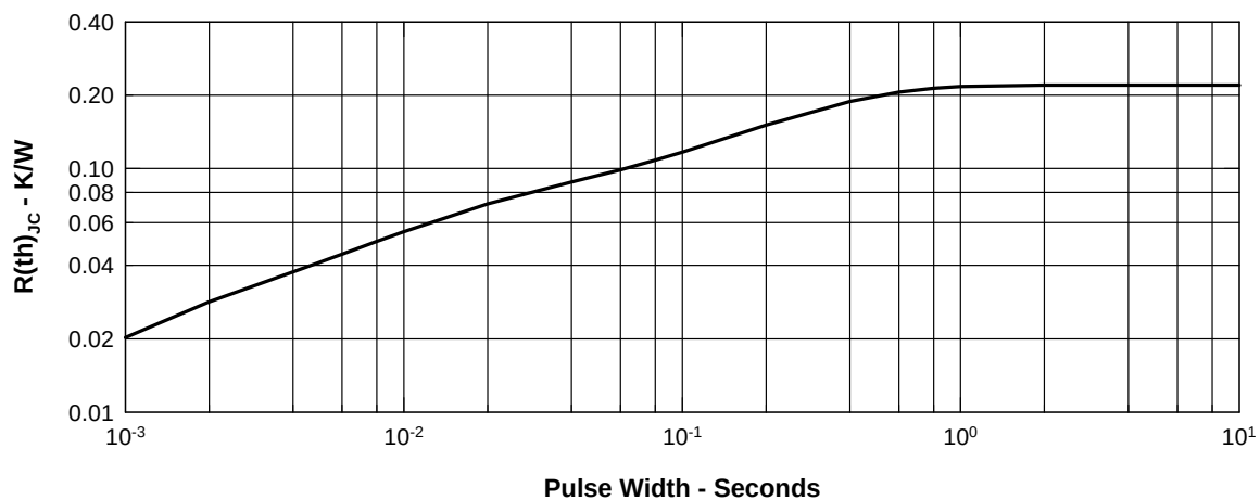
Figure 11. Transient Thermal Resistance
