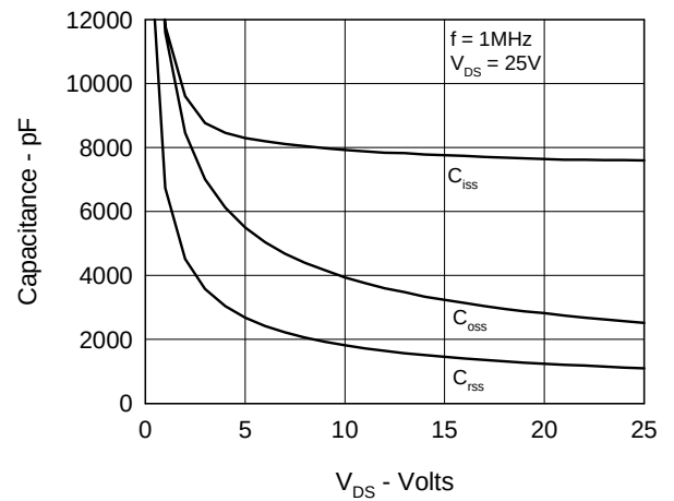
Fig.8 Capacitance Curves
