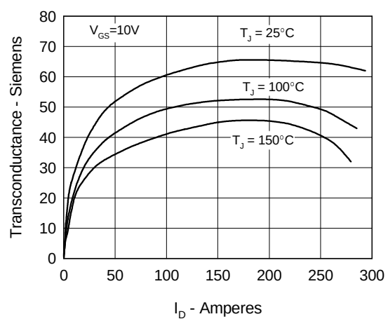
Fig. 6 Transconductance
