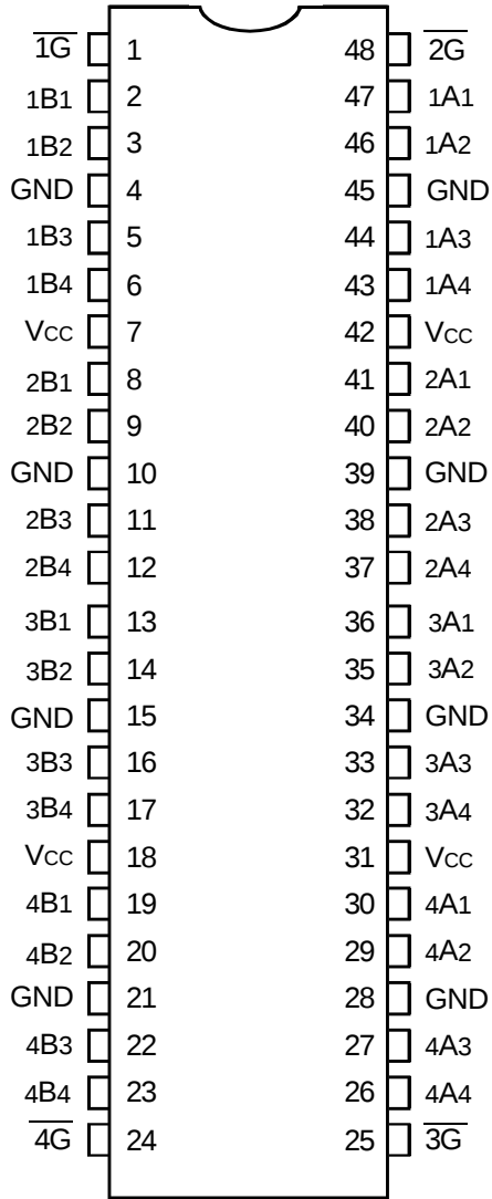
SSOP/ TSSOP TOP VIEW
