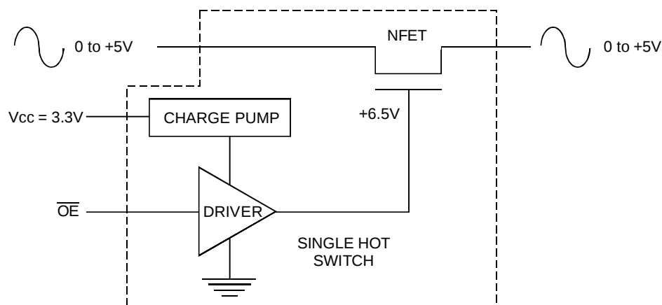
Rail-to-Rail Switching
