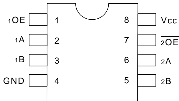
SOIC TOP VIEW
