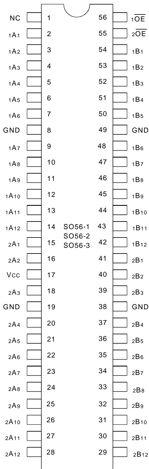
SSOP/TSSOP/TVSOP TOP VIEW
