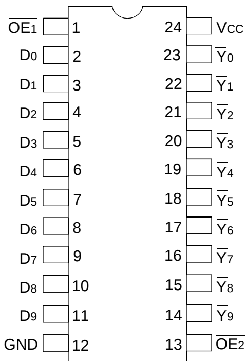
QSOP TOP VIEW
