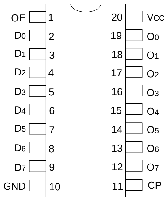
SOIC/ QSOP TOP VIEW
