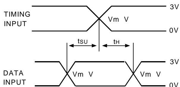
Voltage Waveforms Setup and Hold Times ( V_m = 1.5V for A-Port and 1V for B-Port)
