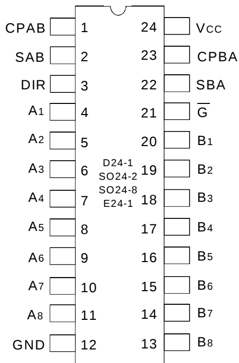
CERDIP/ SOIC/ QSOP/ CERPACK TOP VIEW
