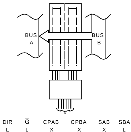
REAL-TIME TRANSFER BUS B TO A
