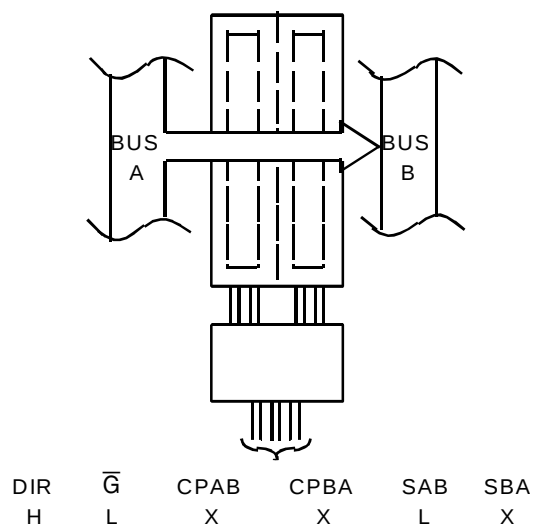
REAL-TIME TRANSFER BUS A TO B
