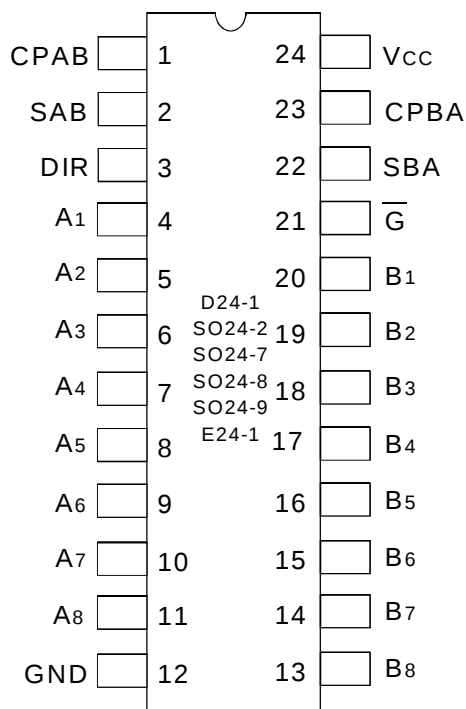
CERDIP/ SOIC/ SSOP/ QSOP/ TSSOP/ CERPACK TOP VIEW
