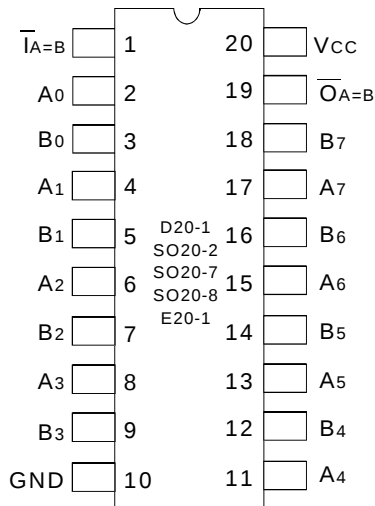
CERDIP/ SOIC/ SSOP/ QSOP/ CERPACK TOP VIEW
