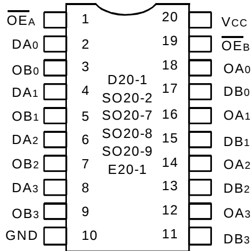
CERDIP/ SOIC/ SSOP/ QSOP/ TSSOP/ CERPACK TOP VIEW
