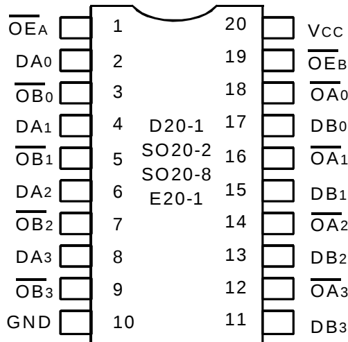
CERDIP/ SOIC/ QSOP/ CERPACK TOP VIEW
