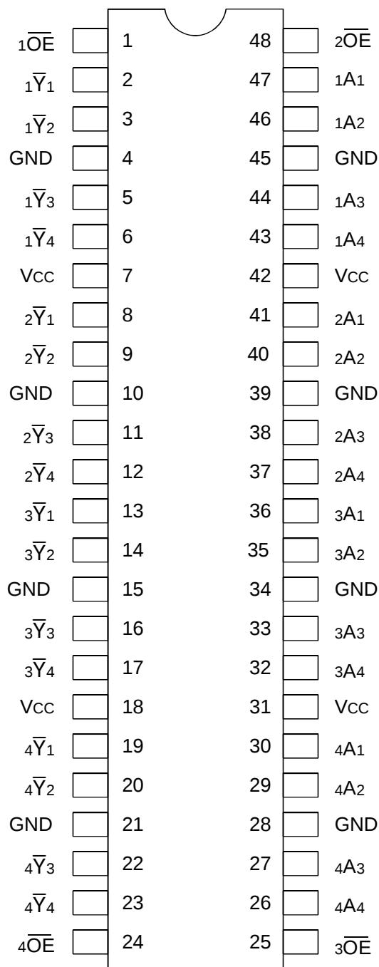
SSOP/ TSSOP/ CERPACK TOP VIEW
