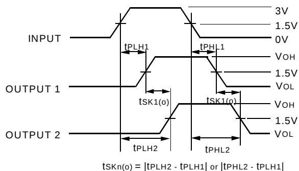
Output Skew - t_{SKn(o)}
