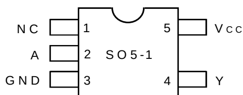
PSOP TOP VIEW
