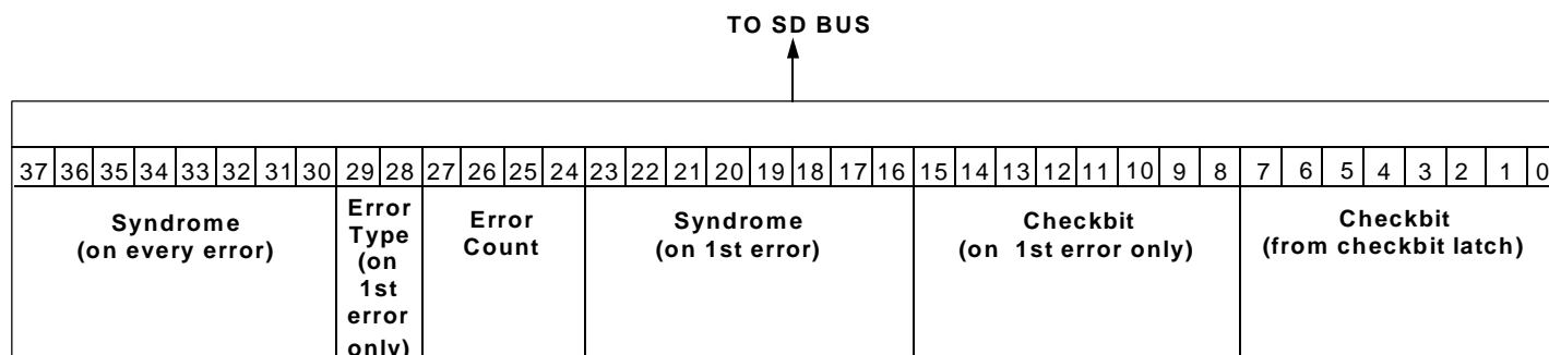
Fig 3. Memory Initialization using Diagnostic Output/Error Data Output Mode
