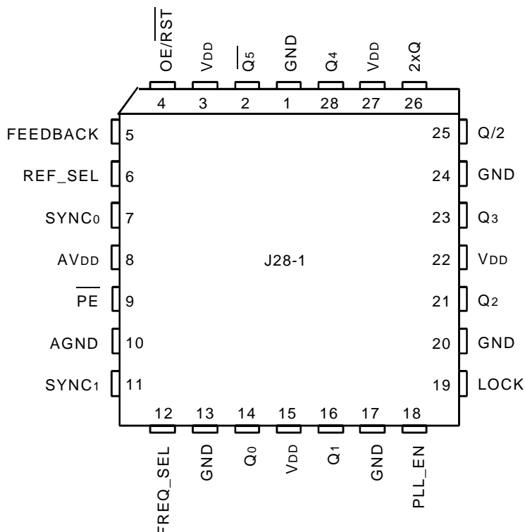
PLCC TOP VIEW
