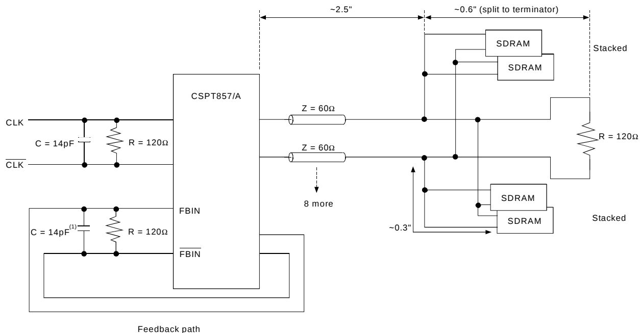
Figure 10. Clock Structure 2
