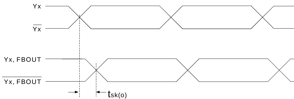
Figure 5. Output Skew
