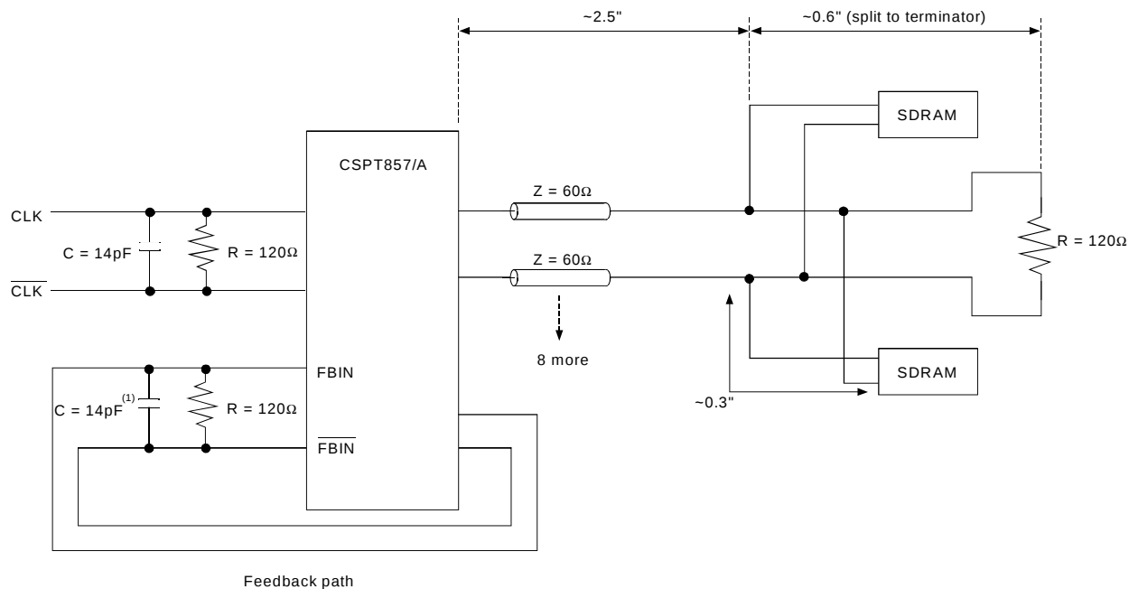
Figure 9. Clock Structure 1
