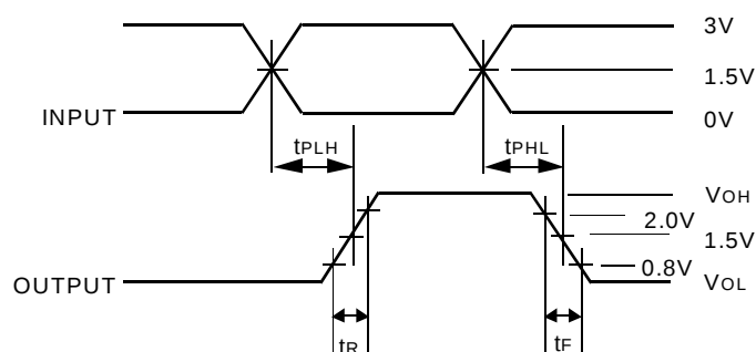
Propagation Delay
