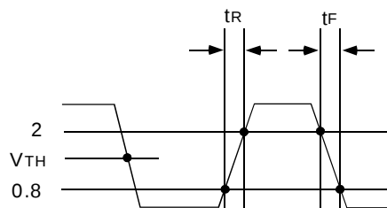
Output Waveform
