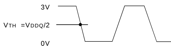
Input Waveform
