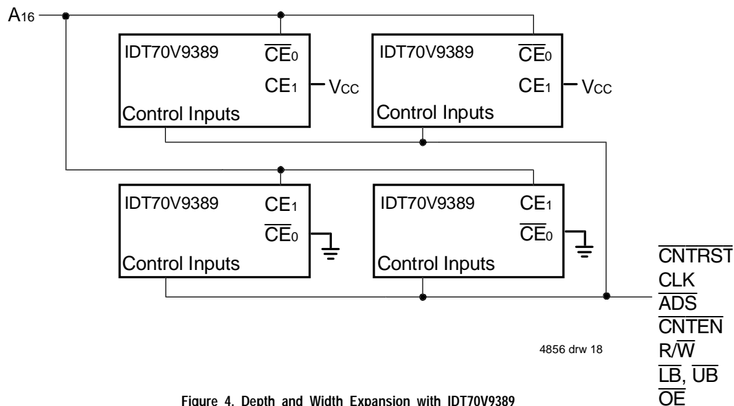
Figure 4. Depth and Width Expansion with IDT70V9389
