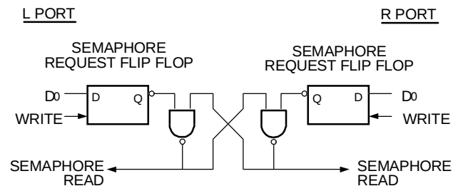
Figure 4. IDT70V658 Semaphore Logic
