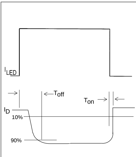
Figure 8. Delay Time Definitions
