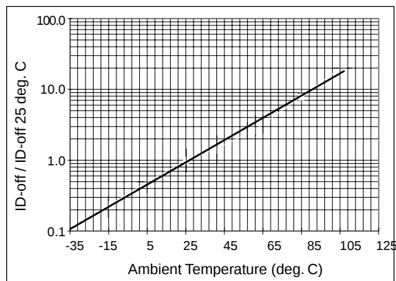
Figure 5. Typical Normalized Off-State Leakage
