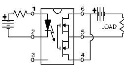
"C" Connection
