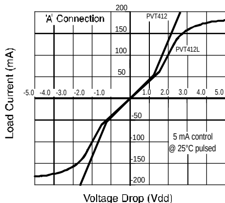
Figure 3. Linearity Characteristics
