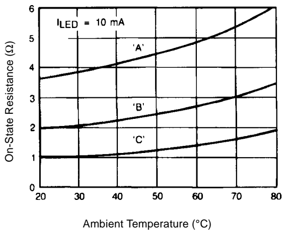
Figure 2. Typical On-Resistance
