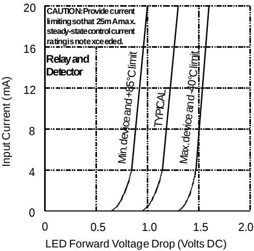
Figure 6. Input Characteristics (Current Controlled)
