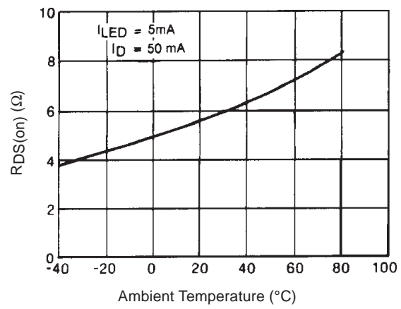
Figure 4. Typical On-Resistance
