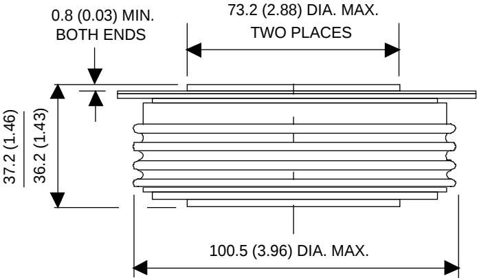
Case Style B-44 (R-PUK) All dimensions in millimeters (inches)
