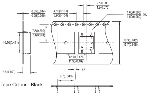
Tape Reel Dimensions for 1B...STRR16/DF...STRR16
