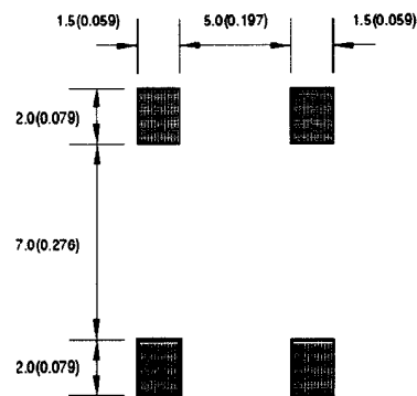
Footprint and Pad Dimensions
