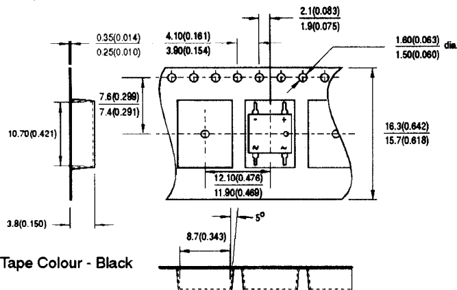
Tape Reel Dimensions for 1B...STRR16/DF...STRR16
