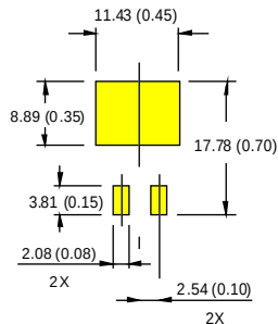
MINIMUM RECOMMENDED FOOTPRINT
