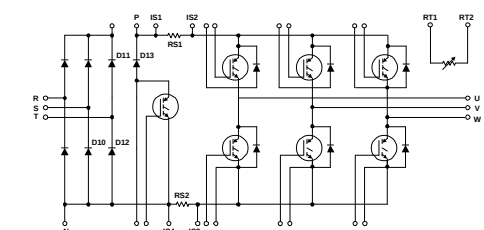
Circuit 4
