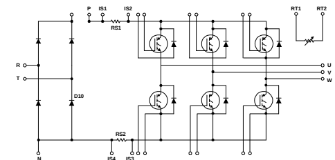
Circuit 1
