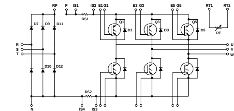
Circuit 3
