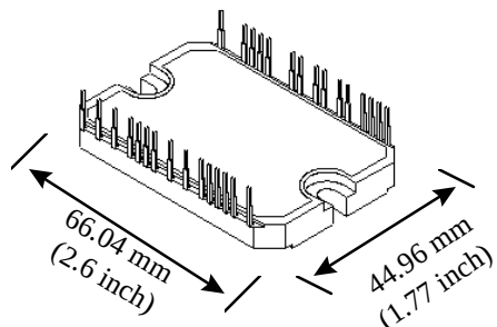
Package 1 (mm)
