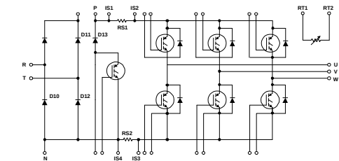
Circuit 2
