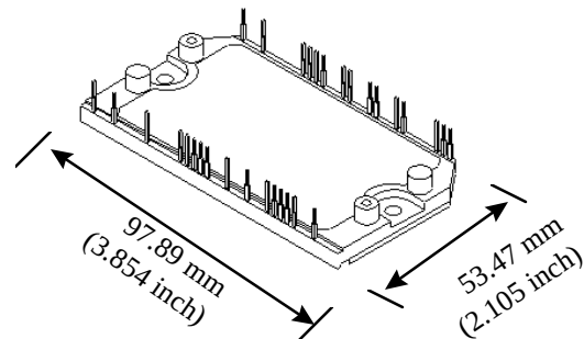
Package 2 (STD)
