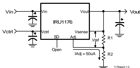
Figure 2 - Typical application of the IRU1176 for programming the output voltage
