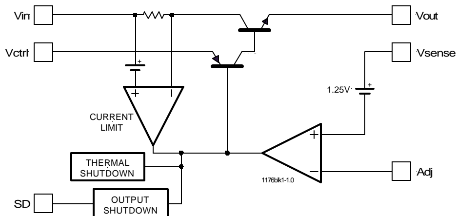
Figure 1 - Simplified block diagram of the IRU1176
