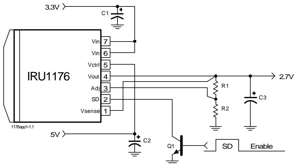
Typical application of IRU1176
