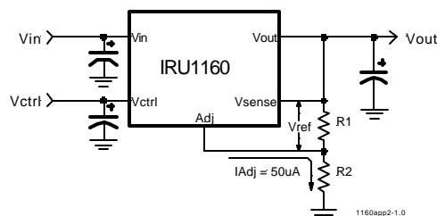
Figure 2 - Typical application of the IRU1160 for programming the output voltage
