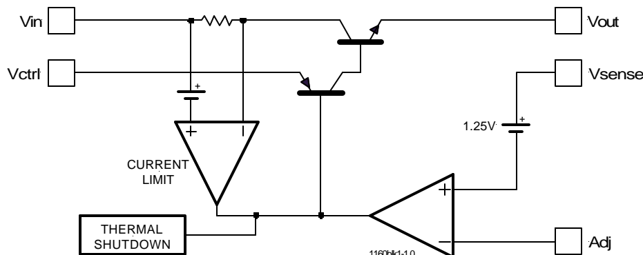
Figure 1 - Simplified block diagram of the IRU1160
