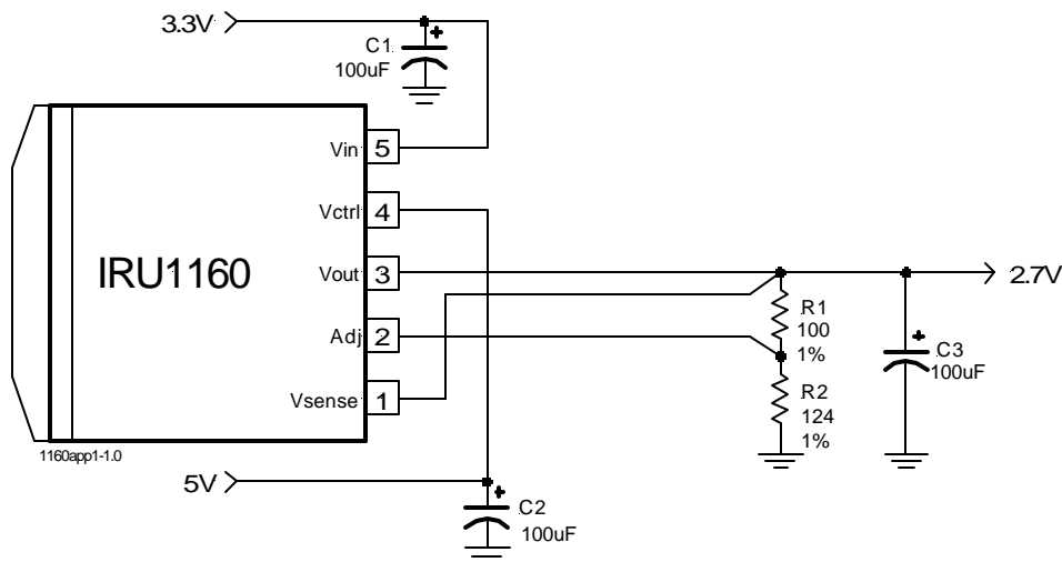
Typical application of IRU1160 in a 3.3V to 2.8V
