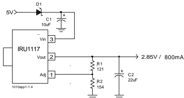
Typical application of IRU1117 in a 5V to 2.85V SCSI termination regulator
