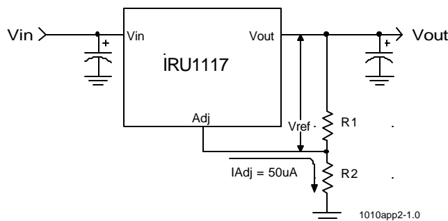
Figure 2 - Typical application of the IRU1117 for programming the output voltage
