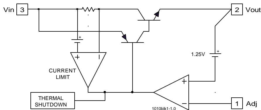
Figure 1 - Simplified block diagram of the IRU1117
