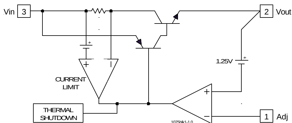
Figure 1 - Simplified block diagram of the IRU1075
