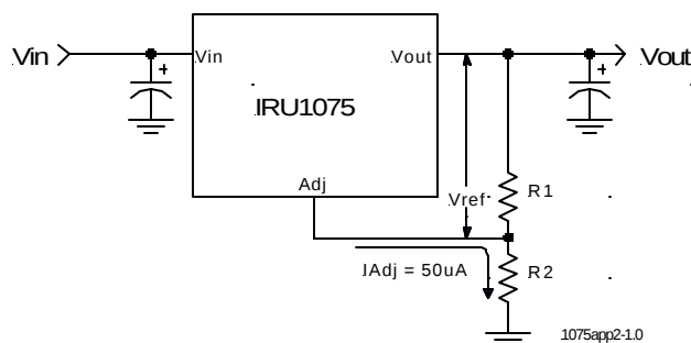
Figure 2 - Typical application of the IRU1075 for programming the output voltage
