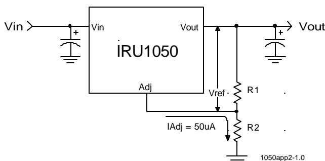
Figure 2 - Typical application of the IRU1050 for programming the output voltage
