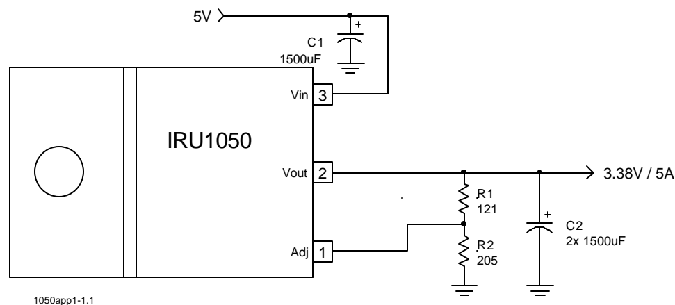
Typical Application of IRU1050 in a 5V to 3.38V regulator designed to meet the Intel P54C™ processors
