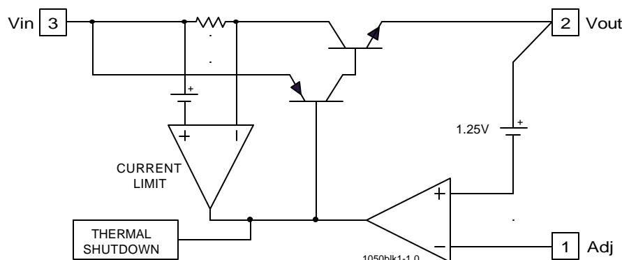
Figure 1 - Simplified block diagram of the IRU1050
