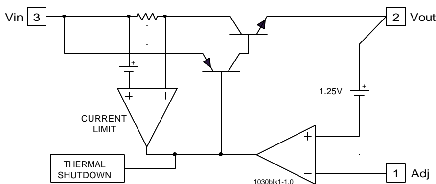
Figure 1 - Simplified block diagram of the IRU1030
