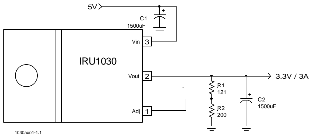
Typical Application of IRU1030 in a 5V to 3.3V regulator
