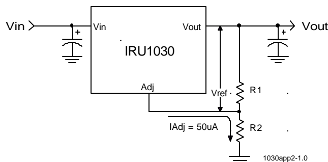
Figure 2 - Typical application of the IRU1030 for programming the output voltage
