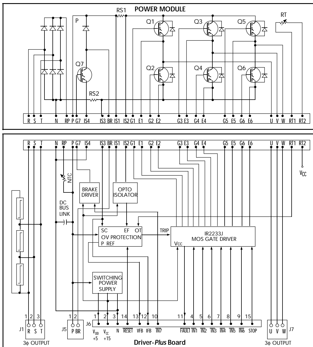
Figure 4. IRPT2062C Basic Architecture
