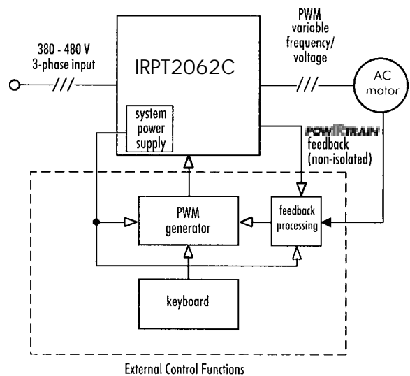
Figure 1. The IRPT2062C POWERTRAIN within a motor control system
