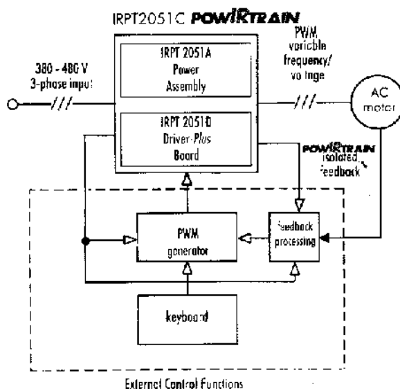
Figure 2. The IRPT2051C POWIRTRAIN within a motor control system
