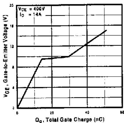
Figure 5b. Typical Gate Charge vs Gate-to-Emitter Voltage
