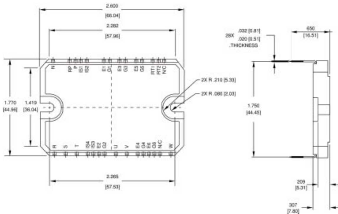
Figure 8a. Package Outline and Mechanical Specifications
