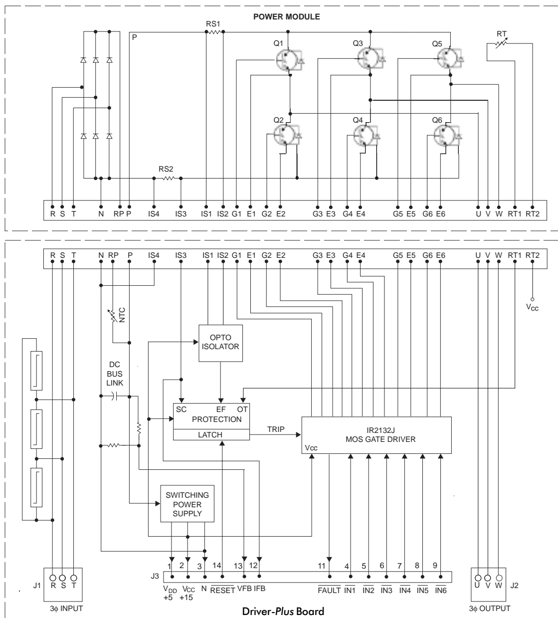
Figure 4. IRPT1057C Basic Architecture
