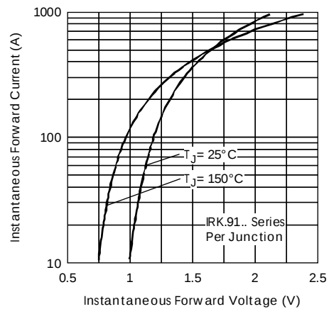
Fig. 10 - Forward Voltage Drop Characteristics
