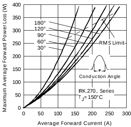
Fig.14-ForwardPowerLossCharacteristics
