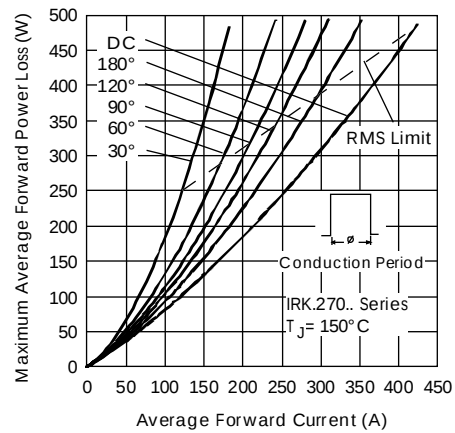
Fig.15-ForwardPowerLossCharacteristics
