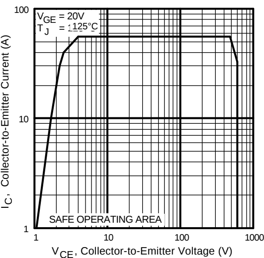
Fig. 12 - Turn-Off SOA
