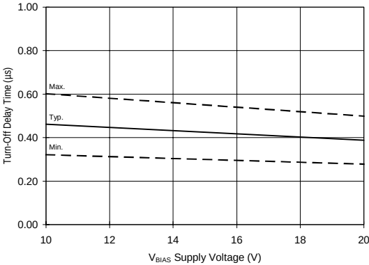
Figure 12B. Turn-Off Time vs. Voltage
