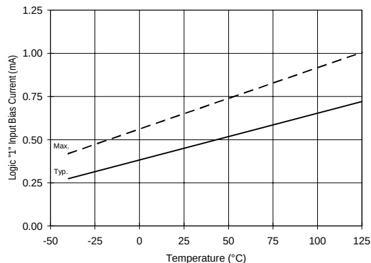
Figure 29A. Logic "1" Input Current vs. Temperature
