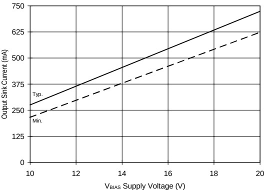
Figure 39B. Output Sink Current vs. Voltage
