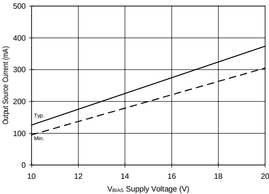
Figure 38B. Output Source Current vs. Voltage
