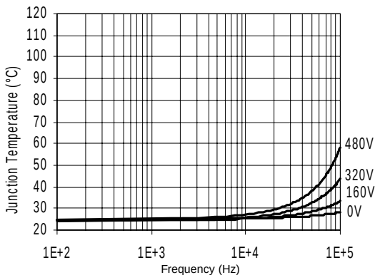
Figure 57. IR2130J/IR2132J T J vs. Frequency (IRGPC40KD2) R GATE = 15W, V CC = 15V
