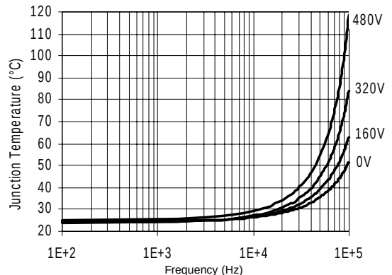
Figure 58. IR2130J/IR2132J T J vs. Frequency (IRGPC50KD2) R GATE = 10W, V CC = 15V
