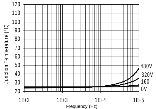
Figure 56. IR2130J/IR2132J T J vs. Frequency (IRGPC30KD2) R GATE = 20W, V CC = 15V
