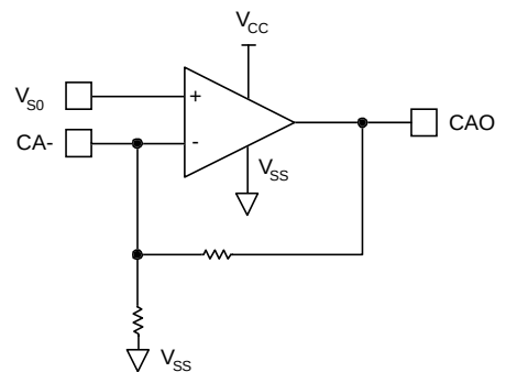
Figure 6. Diagnostic Feedback Operational Amplifier Circuit
