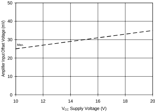
Figure 40B. Amplifier Input Offset vs. Voltage
