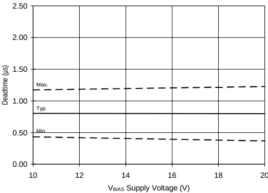
Figure 18D. Deadtime vs. Voltage (IR2132)
