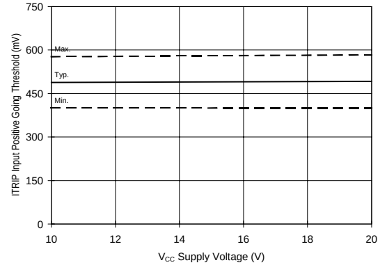
Figure 23B. ITRIP Input Positive Going Threshold vs. Voltage
