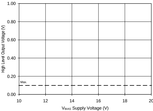
Figure 24B. High Level Output vs. Voltage
