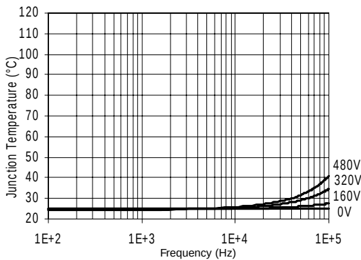
Figure 55. IR2130J/IR2132J T J vs. Frequency (IRGPC20KD2) R GATE = 33W, V CC = 15V
